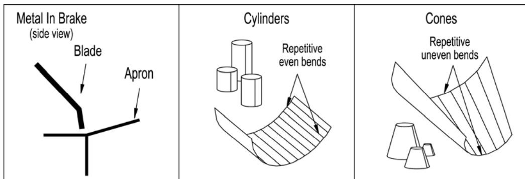
Figure 10 – Radius Bending
